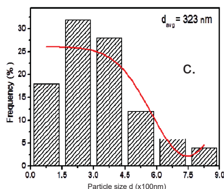
Fig. 3 Particle size distribution of BiOBr-1 (a), BiOBr-2 (b), and BiOBr-3 (c)
