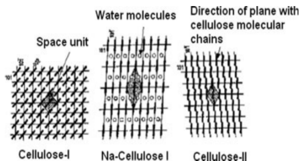
Fig. 2 Lattice structure of cellulose I and cellulose II [21]
