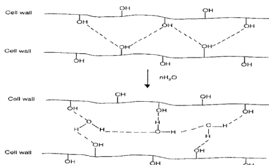
Fig. 1 schematic illustration of the swelling process in cellulose [37]
