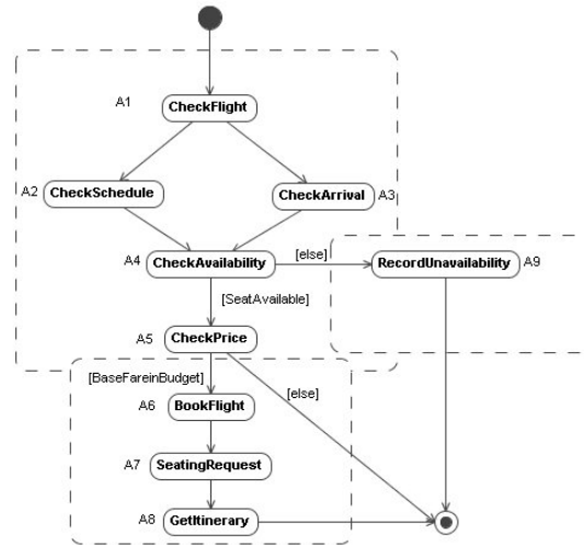
Fig. 4 A design with three process components
