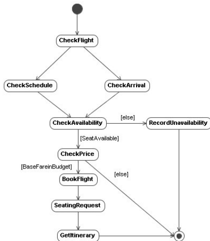
Fig. 3 Business process of flight reservation domain
