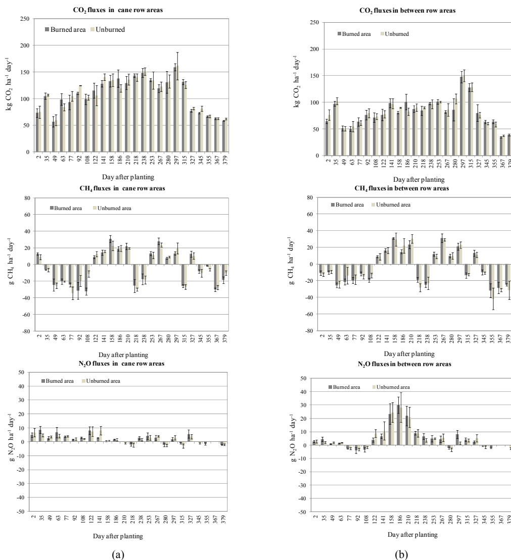
Fig. 3 Daily flux of \text{CO}_2 , \text{CH}_4 , and \text{N}_2\text{O} from (a) the sugarcane plant-row soil and (b) the spaces between-rows soils unburned the burned and unburned sugarcane plantation areas over 379 DAP
