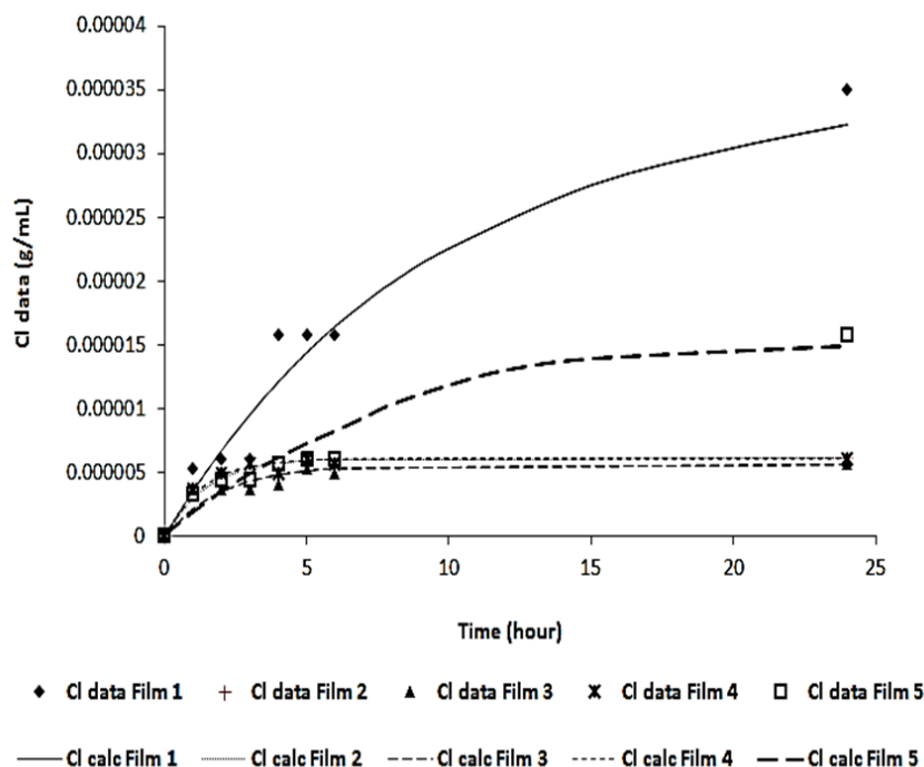
Fig. 5 Comparison between CI data and CI Calculate with Loading Time 12 hours
