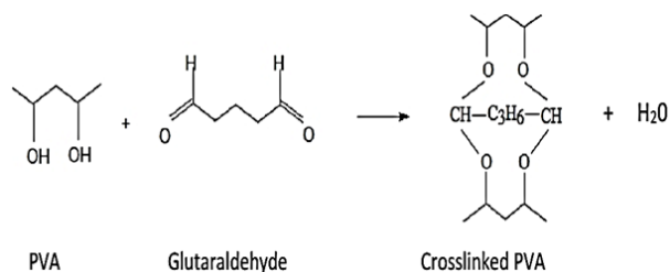
Fig. 4 Structure of PVA Crosslinked
