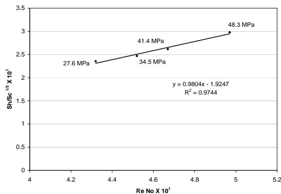
Fig. 2 Correlation between \text{Sh}/\text{Sc}^{1/3} versus Re No constant temperature of 50 ^{\circ}\text{C} and pressures ranging from 27.6 MPa to 48.3 MPa
