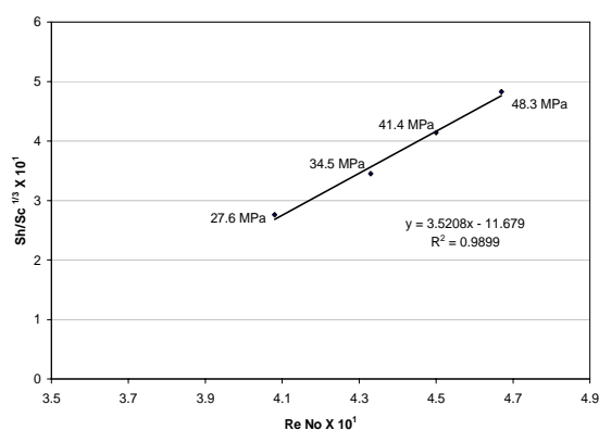
Fig. 3 Correlation between \text{Sh}/\text{Sc}^{1/3} versus Re No at constant temperature of 60 ^{\circ}\text{C} and pressures ranging from 27.6 MPa to 48.3 MPa
