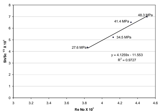
Fig. 4 Correlation between \text{Sh}/\text{Sc}^{1/3} versus and Re No at constant temperature of 70 ^{\circ}\text{C} and pressure ranging from 27.6 MPa to 48.3 MPa
