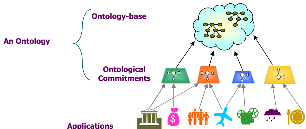
Figure 1: Knowledge organization in DOGMA approach
