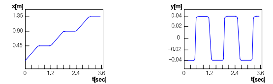
(b) ZMP trajectory in the sagittal plane (c) ZMP trajectory in the lateral plane Fig. 8 Human's COG and ZMP trajectory
