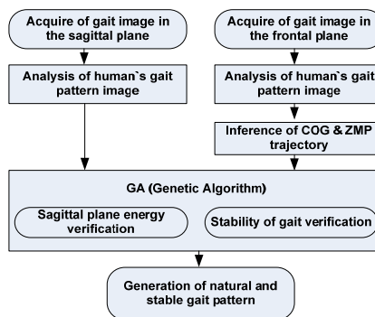
Fig. 11 Flow of the proposed algorithm
