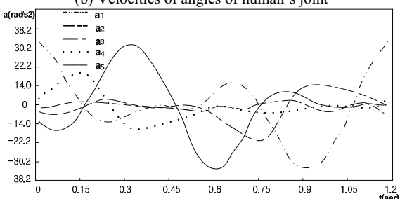
(a) Angles of human's joint (b) Velocities of angles of human's joint (c) Accelerations of angles of human's joint Fig. 9 Rotation components of Human's joints during one period gait
