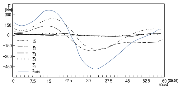
Fig. 10 Human's calculated torques
