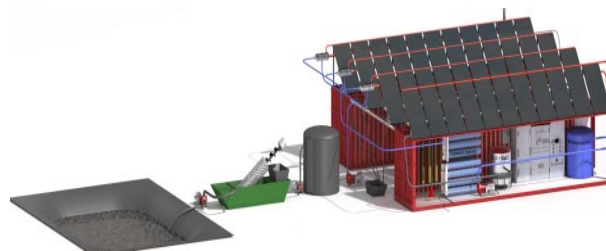
Fig. 2 LEACHLESS prototype
