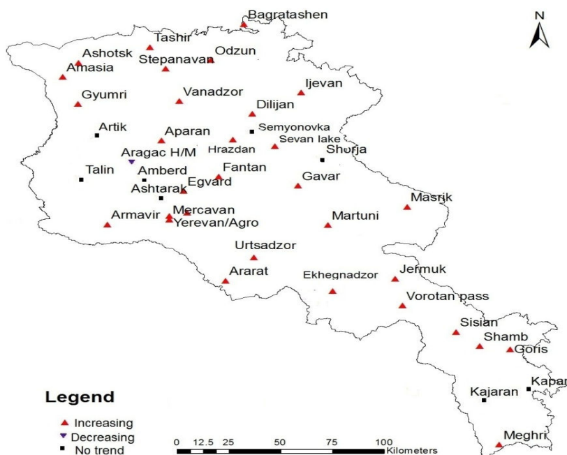
Fig. 1 Rank correlation tests results (point data)
