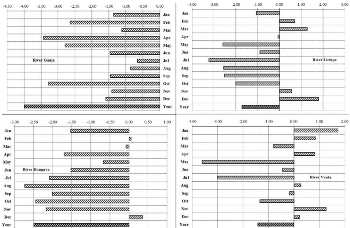
Fig. 7 Trends of long-term seasonal changes of N_{total} in waters of rivers of Latvia (Gauja, Lielupe, Daugava and Venta 1980 – 2015) after Man-Kendall test criteria
