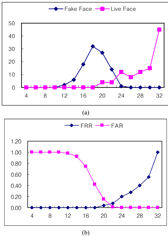
Fig. 6 (a) Distribution of liveness scores (b) ROC curve
