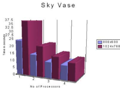
Fig. 4 Results of rendering skyvase.pov on a cluster with varying number of processing slave nodes
