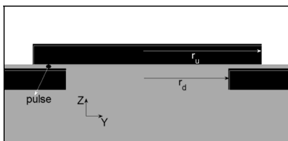
Fig. 4 The y - z plane of the structure which is taken at the center of the x -axis of the simulation cell showing a profile of the two disks. The black (gray) area is silicon ( \text{Si} ). White color represents air
