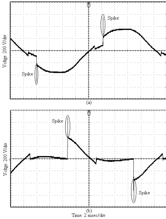
Fig. 2 Effect of firing angle on voltage waveform: (a) \alpha = 30^\circ and (b) \alpha = 90^\circ
