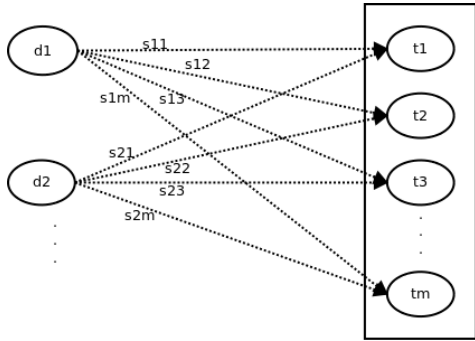
Fig. 1 topic vectors are consists of topic belongingness of each document (d for documents, t for latent topics, and s for document-topic similarity)
