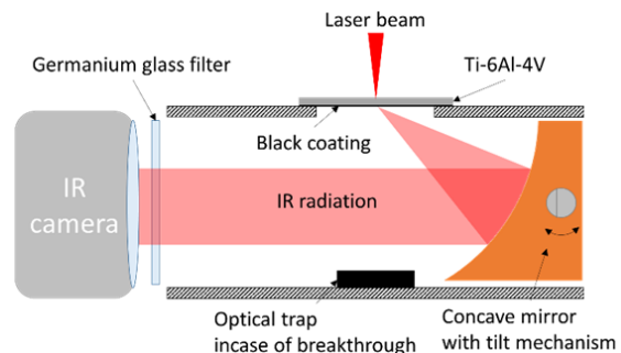
Fig. 2 IR thermography setup
