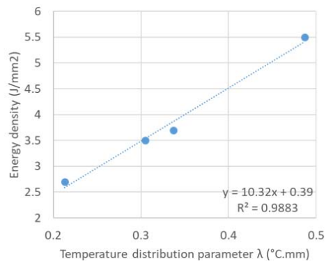
Fig. 7 Correlation between \lambda and energy density
