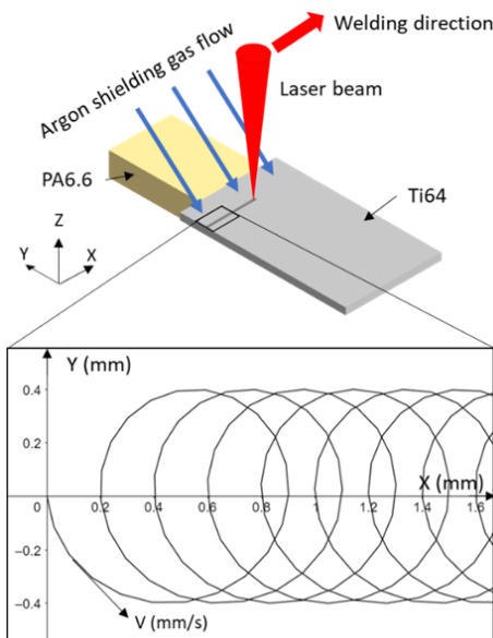
Fig. 1 Laser welding setup
