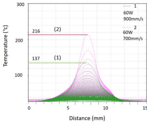
Fig. 4 Effects of varying beam speed on spatial temperature profile
