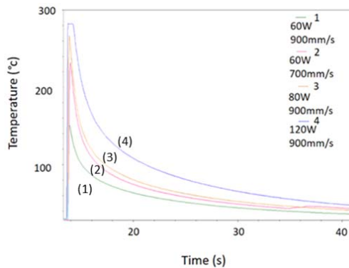
Fig. 5 Temporal thermography
