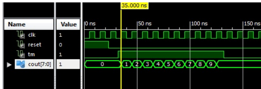
Fig. 11 Simulation result of transmission signal in iSim
