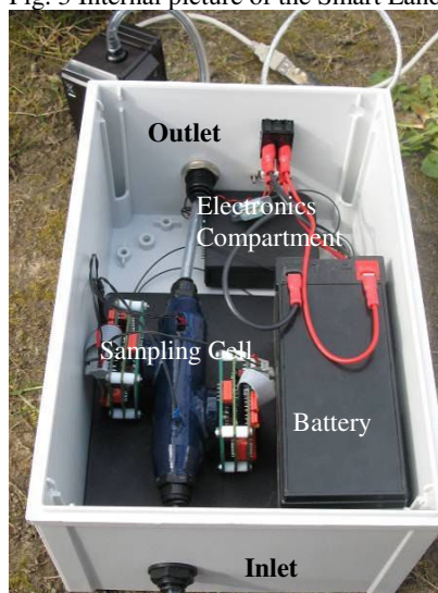
Fig. 3 Internal picture of the Smart Landfill Unit
