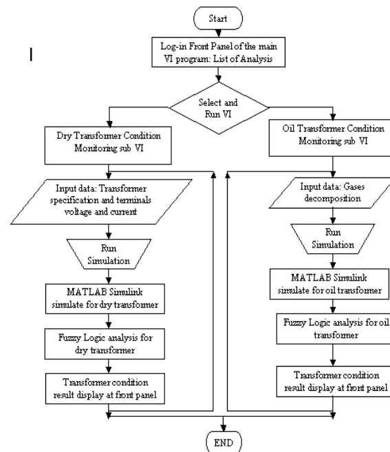
Fig. 1 Structure of the system
