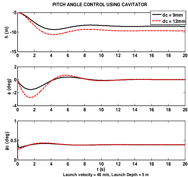
Fig. 14 Pitch angle control using cavator
