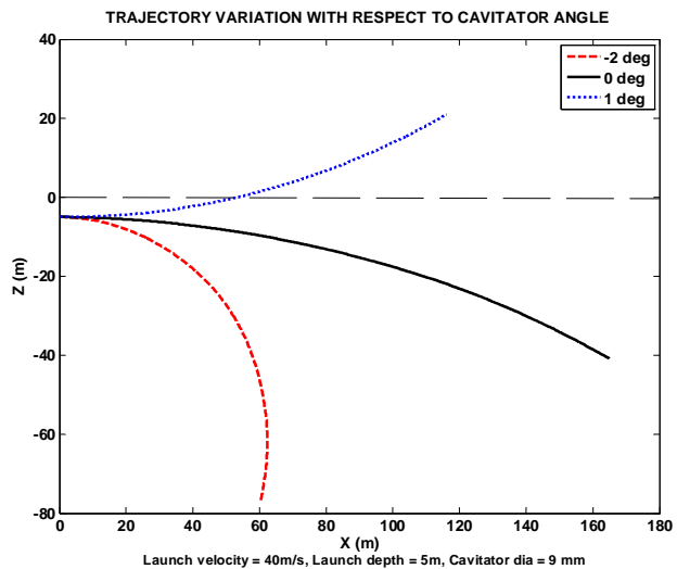
Fig. 9 Trajectory variation with cavitator angle
