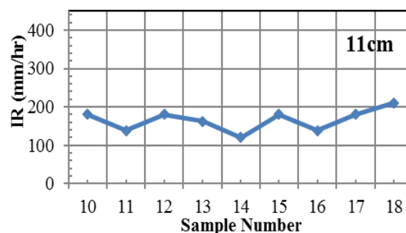
Fig. 3 Infiltration rates for 11cm head
