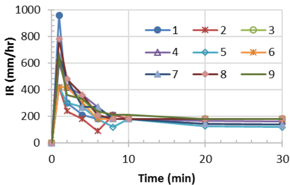
Fig. 4 Attainment of steady-state infiltration rates
