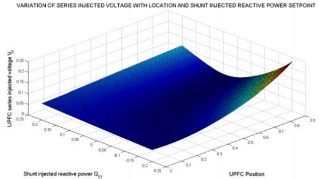
Fig. 8. Variation of series injected voltage V_B with reactive power Q_{Et} setpoint and location variation
