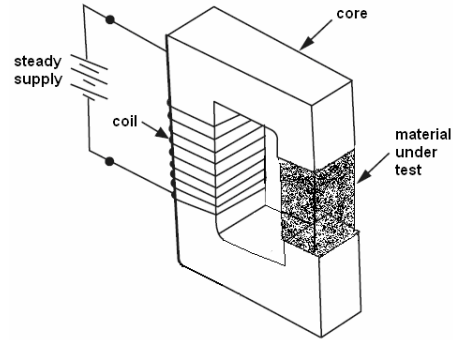
Fig. 3 Structure of electromagnetic field exciter
