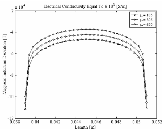
Fig. 5 Magnetic induction deviation for three values of magnetic relative permeability and electrical conductivity equal to 6 \cdot 10^3 (S/m)
