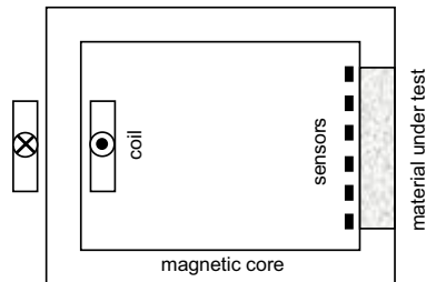
Fig. 4 Arrangement for the measurements
