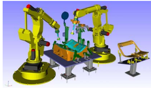
Fig. 3 Robot cell layout at Saab Automobile AB
