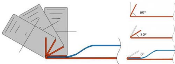
Fig. 2 Three steps in the roller hemming process
