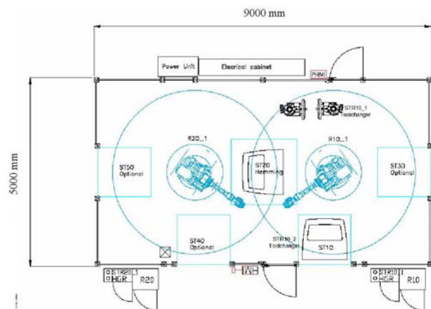
Fig. 6 Robot cell layout and operability region
