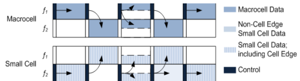
Fig. 2 ICI coordination based on carrier aggregation
