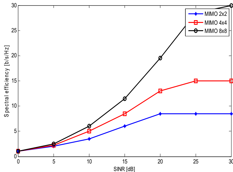
Fig. 8 Spectral efficiency evaluation according to MIMO configuration
