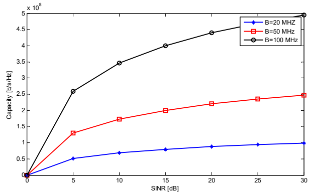
Fig. 4 LTE-Advanced capacity depending on bandwidth
