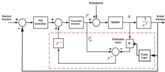
Fig. 7 Proposed AFCFL scheme
