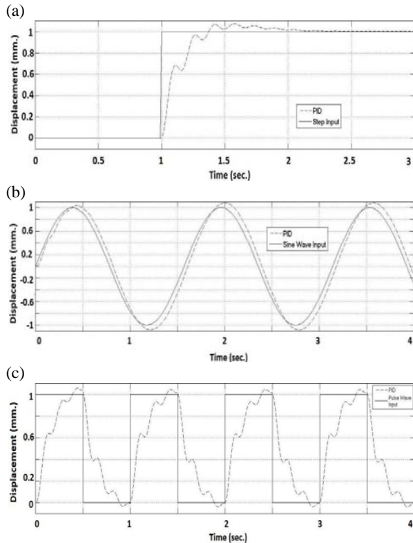
Fig. 3 Performance of PID controller for (a) step, (b) sine wave, and (c) square input functions
