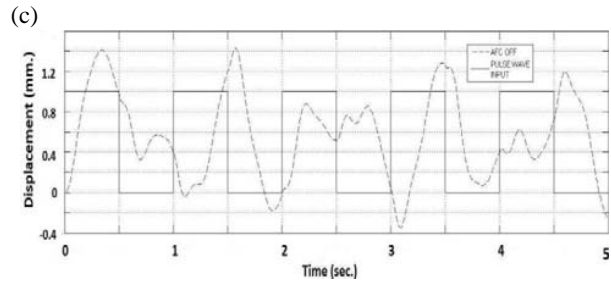
Fig. 8 Effect of harmonic disturbance on system response for PID controller only (AFCFL – OFF) for various input conditions
