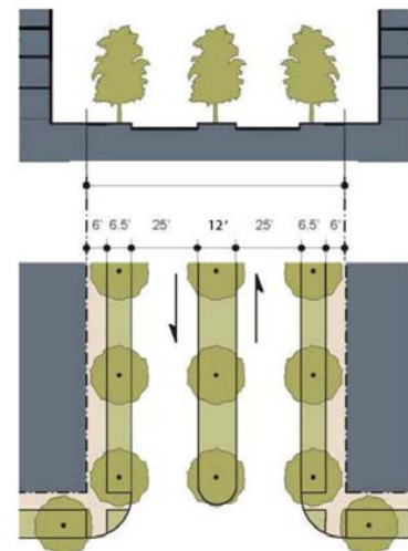
Fig. 17 Street dimensions based on the Hudson Farm Master Plan
