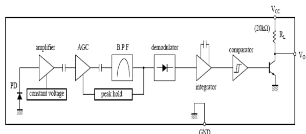
Fig. 4 Block Diagram Of Receiving Section of PNA4602M
