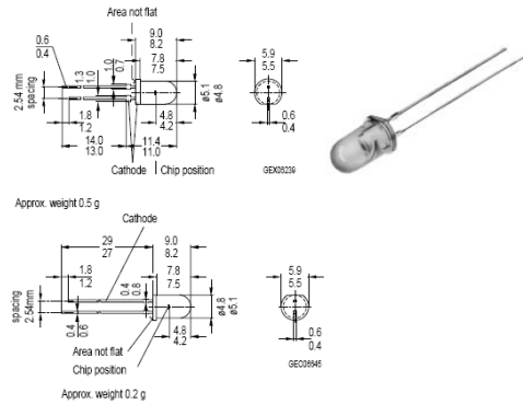
Fig. 1 Infrared Transmitter [LD271H]
