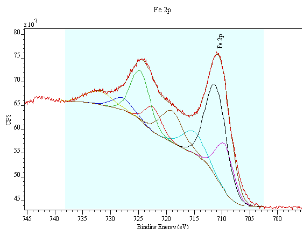
Fig. 3 XPS spectrum of the surface of the fractured siderite sample at 475^\circ\text{C}
