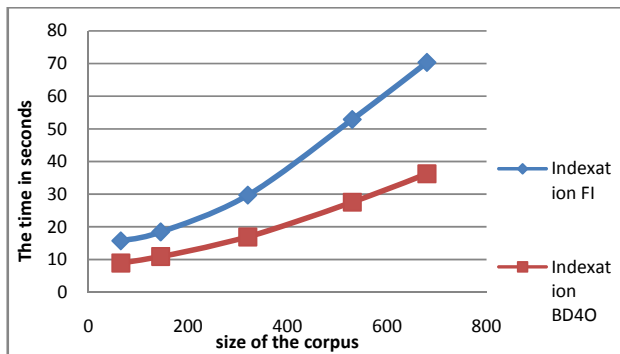
Fig. 5 Comparison of indexing time in db4o and the inverted file
