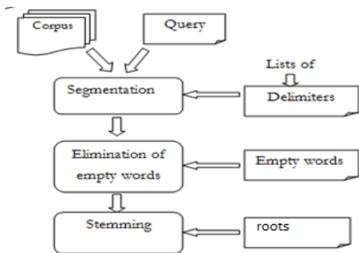
Fig. 4 Phases of indexing of proposed system
