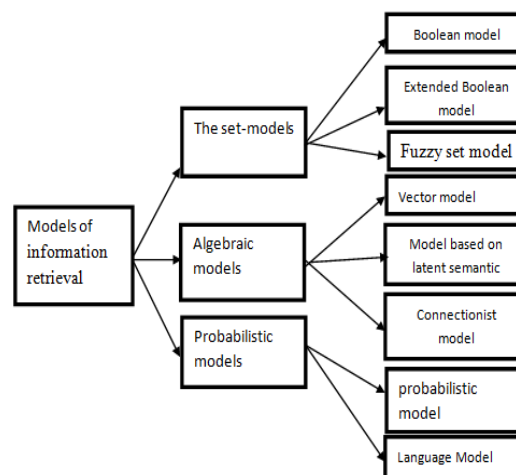
Fig. 3 The various models of information retrieval
