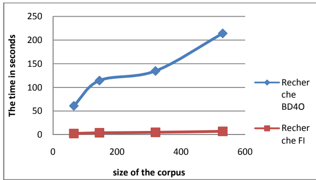
Fig. 7 Comparison of search time in the BD4O and FI size of the corpus
