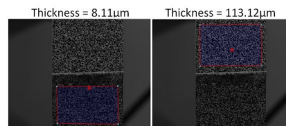
Fig. 5 Area of interest of both coating thickness steps
