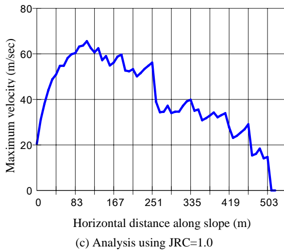
Fig. 4: Influence of the maximum velocity by surface roughness during a rockfall.
