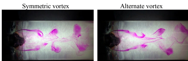
Fig. 5 Modes of vortex shedding for Body B8 at Re_D = 900
