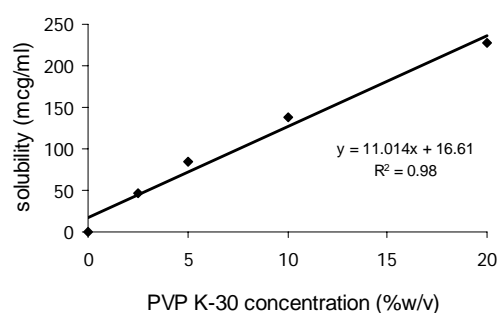
Fig. 1 Solubility profile of curcumin in various concentrations of PVP K-30 at 37±0.1°C
