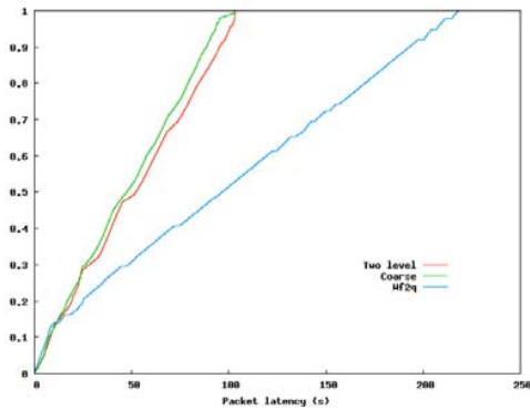
Fig. 22. CDF - Packet latencies: G3
