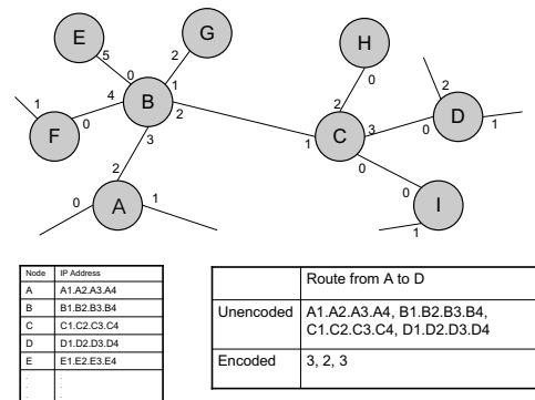
Fig. 3. Path encoding: example graph
