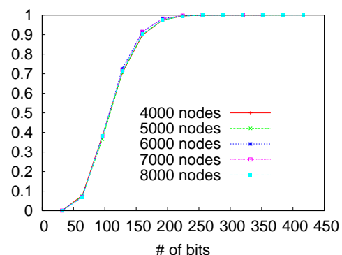
Fig. 6. CDF: WITHOUT encoding
