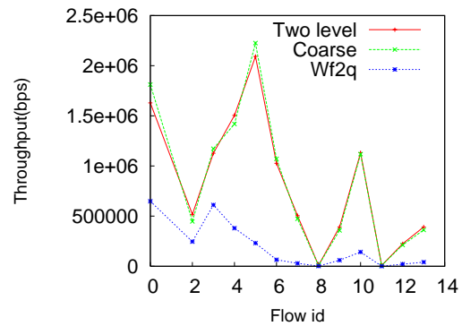
Fig. 19. Per-flow throughput: G3
