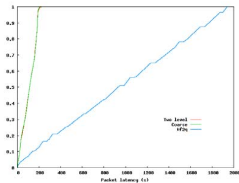
Fig. 20. CDF - Packet latencies: G1
