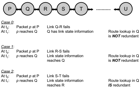
Fig. 2. Redundancy: example topology
