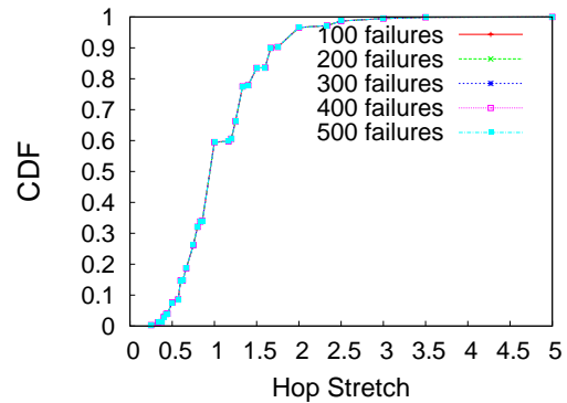
Fig. 8. Effect of number of failures
