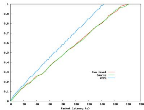
Fig. 21. CDF - Packet latencies: G2
