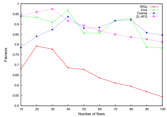
Fig. 13. Comparison of fairness
