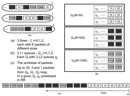
Fig. 12. Two level AFQ scheduling
