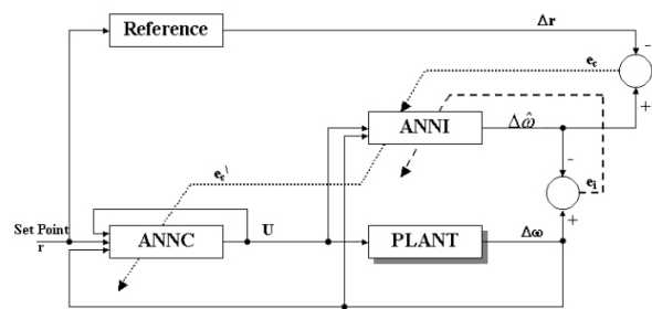
Fig. 3 ANN-PSS architecture
