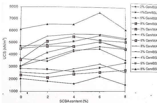
Fig. 13 Variation of UCS with SCBA content at the different compaction energy levels [19]
