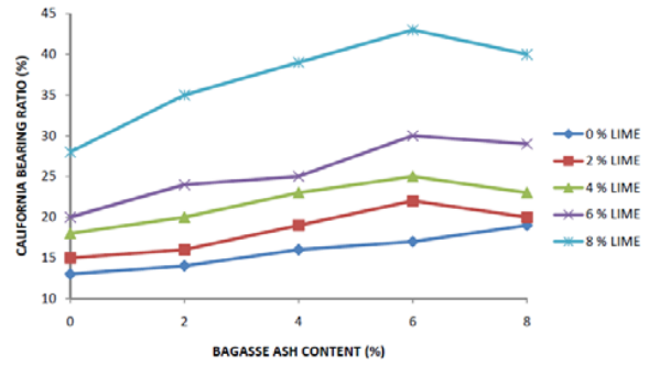
Fig. 18 Variation of unsoaked California bearing ratio of lime stabilized lateritic soil with bagasse ash content [25]
