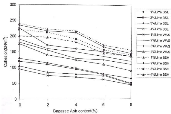
Fig. 10 Variation of cohesion with bagasse ash content for the different compaction energy levels [13]
