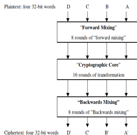
Fig. 1 High-level structure of MARS encryption procedure [5]
