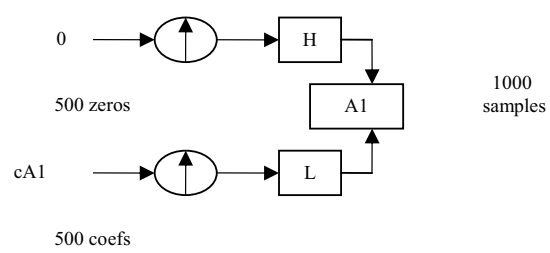
Fig. 3 Wavelet reconstruction from approximation and detail vectors
