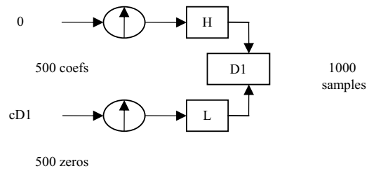
Fig. 4 Wavelet reconstruction for detail vector
