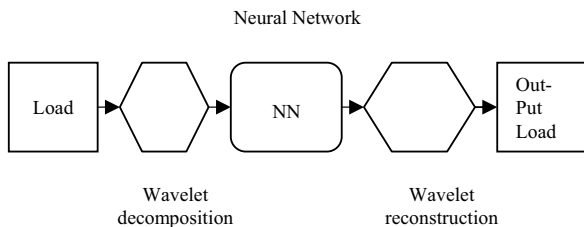
Fig. 7 Neural network model for time series forecasting
