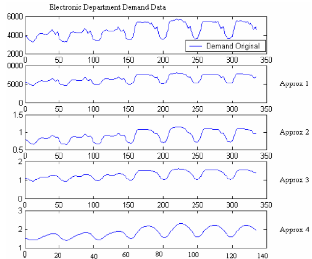
Fig. 13 Comparison of Different Resolution Levels
