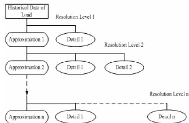
Fig. 11 Wavelet decomposition process
