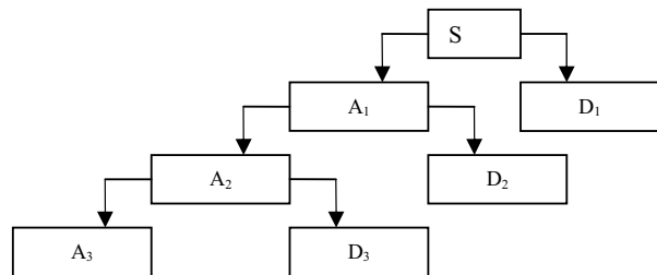
Fig. 5 Wavelet reconstruction from approximation and detail vectors
