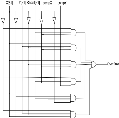
Fig. 8 Overflow Design
