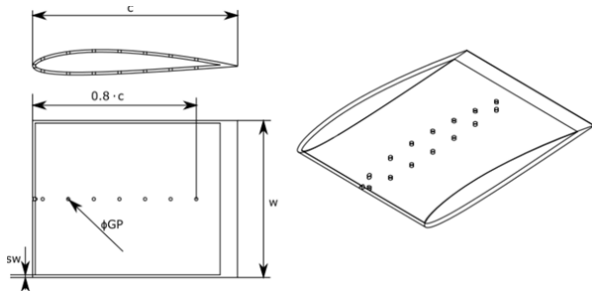
Fig. 2 Airfoil specifications
