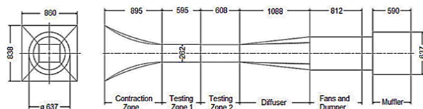
Fig. 1 Wind tunnel dimensions
