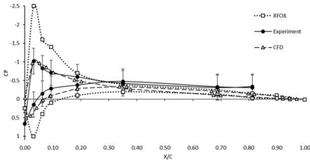
Fig. 6 \alpha = 5 degrees
