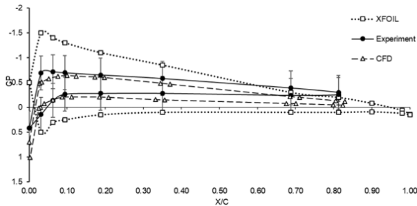
Fig. 7 \alpha = 10 degrees
