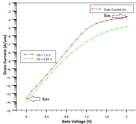
Fig. 4 Sub-threshold I_D - V_{GS} curve for Vertical DG-MOSFET device
