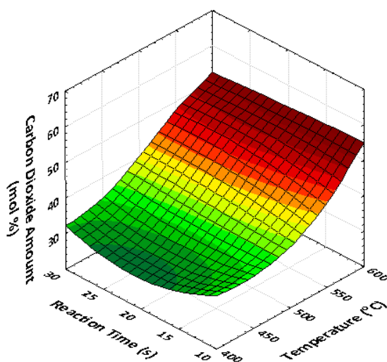
Fig. 7 The change of carbon dioxide amount with temperature and reaction time
