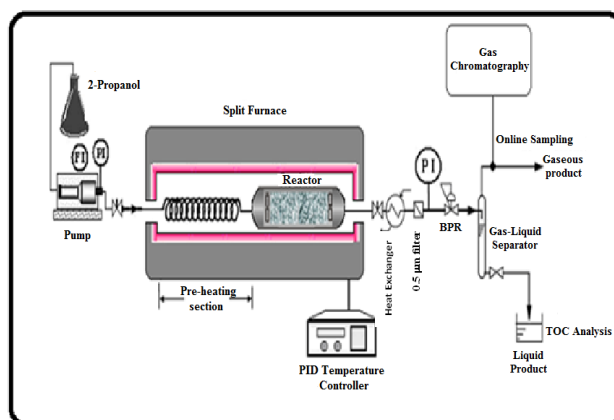
Fig. 3 Schematic demonstration of the experimental setup
