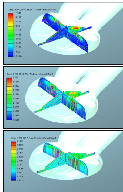
Fig. 2 Turbulent velocity for engine speed of 2000rpm, 4000rpm, and 5000rpm during -345 deg. crank angle intake stroke
