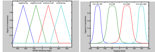
(a) MEMS sensor MF
