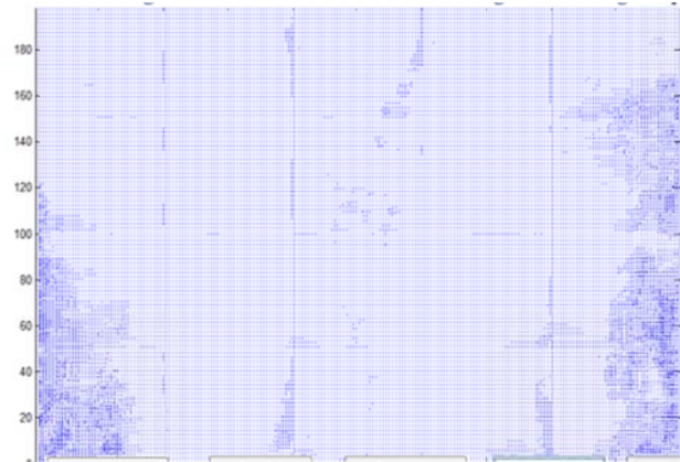
Fig. 3 Optical Flow
