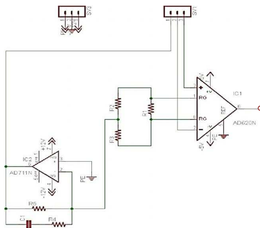
Fig. 2 Bio-Amplifier
