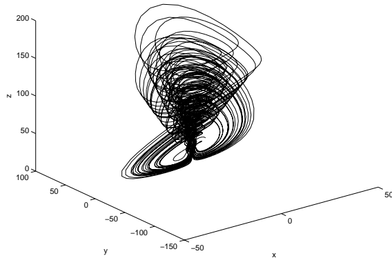
Fig. 1. Chaotic attractor of system (3) with a = 20 , b = 2 , c = 28 and d = 1 .
