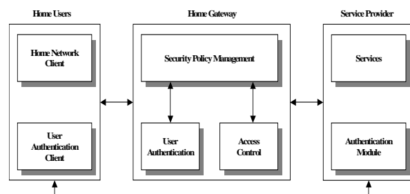
Fig. 1 Components for Home Network Security
